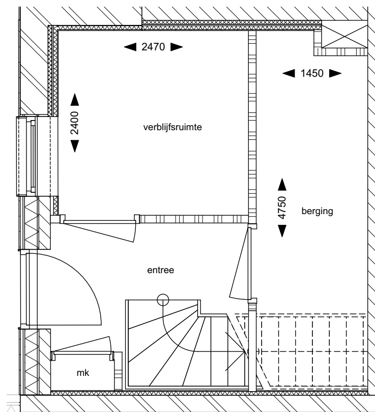
begane grond P=0
